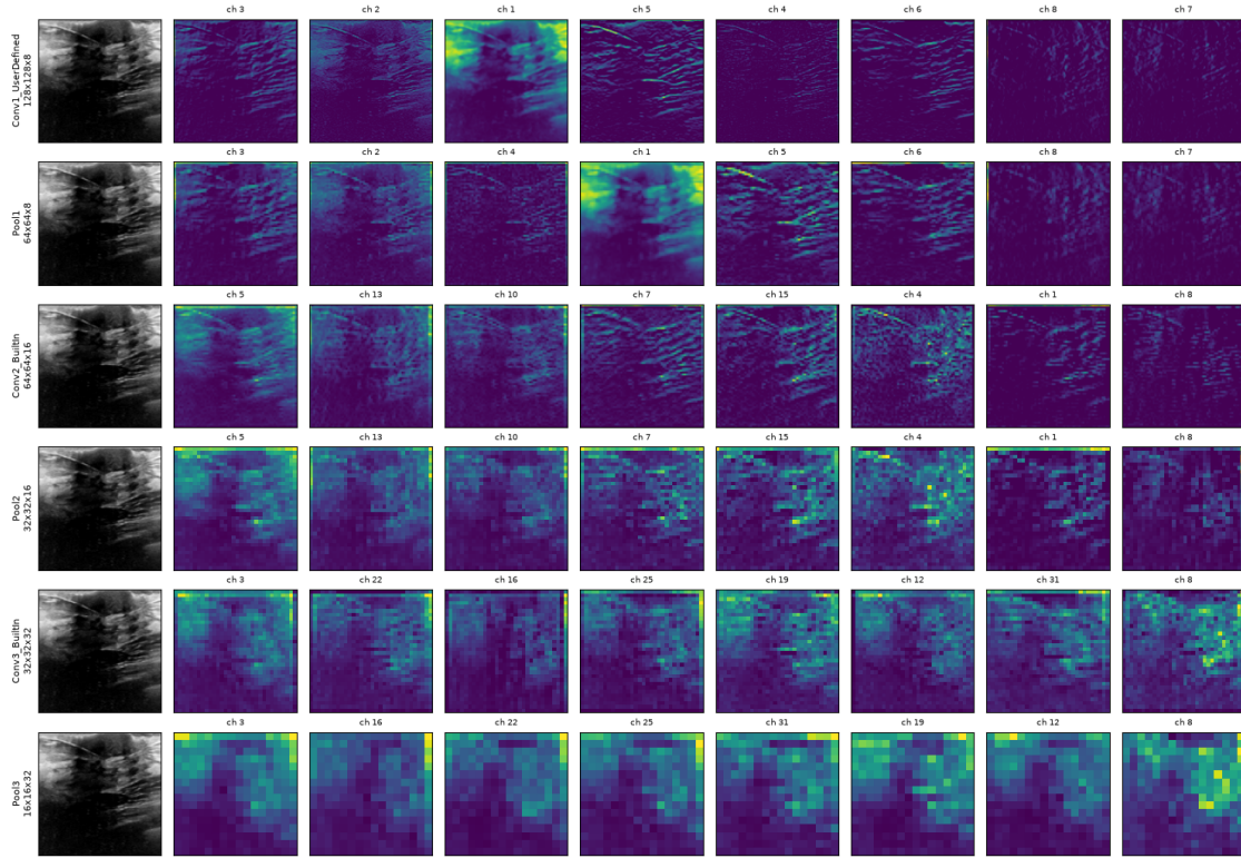
Ultrasound: top 8 channels after every conv and pool layer
