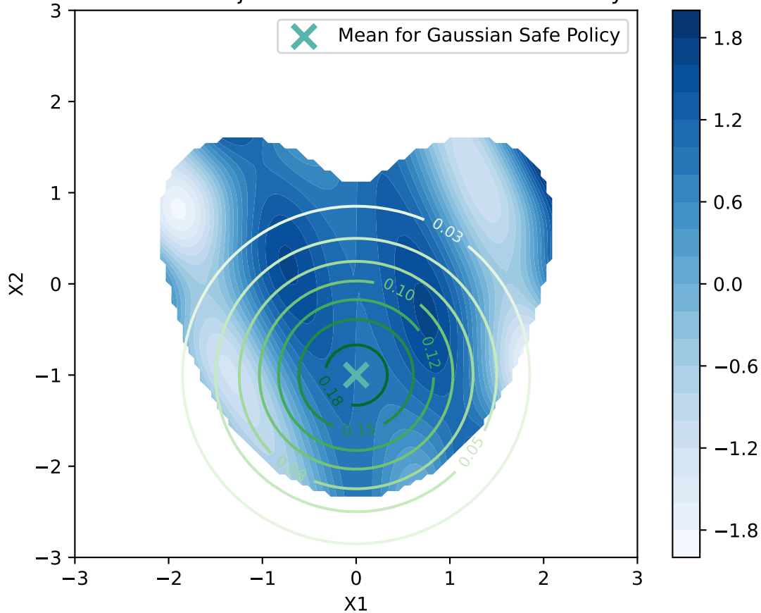
Townsend Objective with Gaussian PDF Overlay
