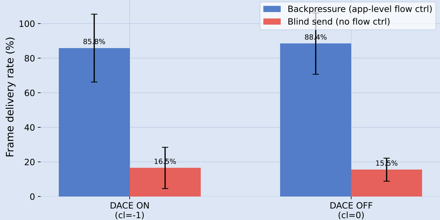
Frame Delivery: Backpressure vs Blind Send (640×360 @ 5fps 500kbps)
