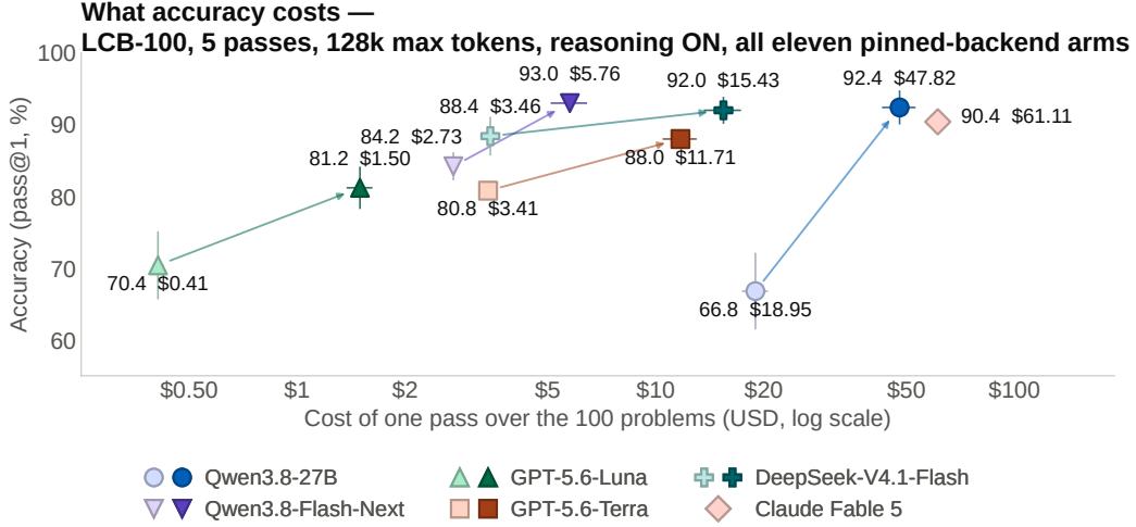
Fig. 3 Cost against accuracy. One point per arm; an arrow runs from the single call to the manager of each model that has both. x is dollars for one pass over the 100 problems (log scale), y is pass@1; the bar through each point is the 95% CI across the 5 passes ( t , df = 4 ). Light fill = single call, dark = with manager; marker shape is the model.
