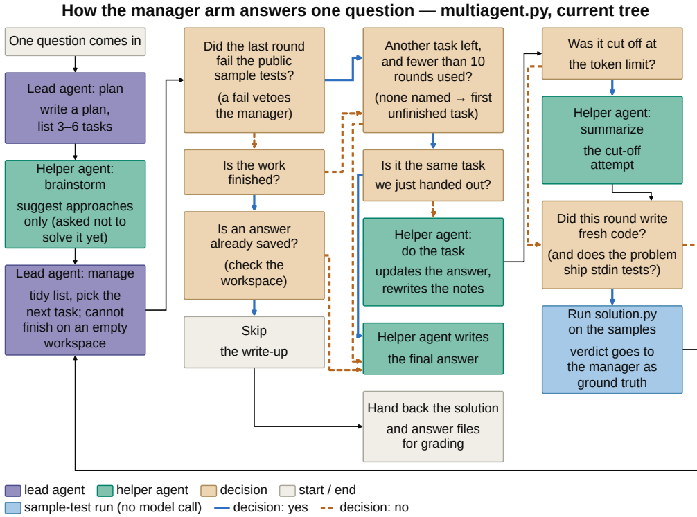
Fig. 1 Manager–worker control flow , as the v2 scaffold runs it. Boxes labelled with an agent are model calls in a fresh context; the decisions, the start and end nodes, and the sample-test run are harness logic and call no model. The boxes absent from the original scaffold are the verifier of step 5 and the cut-off summarizer.
