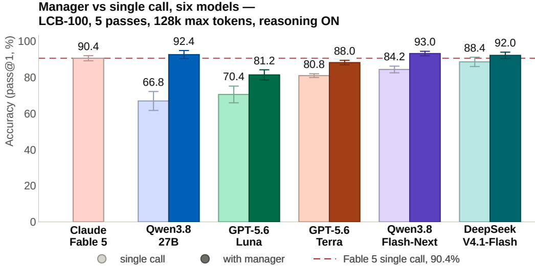
Fig. 2 Manager vs. single call. The scores from Table 1 in a graph. Bars are pass@1 on the same 100 problems, the line through each the 95% CI across the 5 passes ( t , df = 4 ). The left bar of each pair is the single call, light; the manager is beside it, dark; colour is the model. Fable 5 ran single-only, so it has one bar, which the dashed rule carries across the chart.
