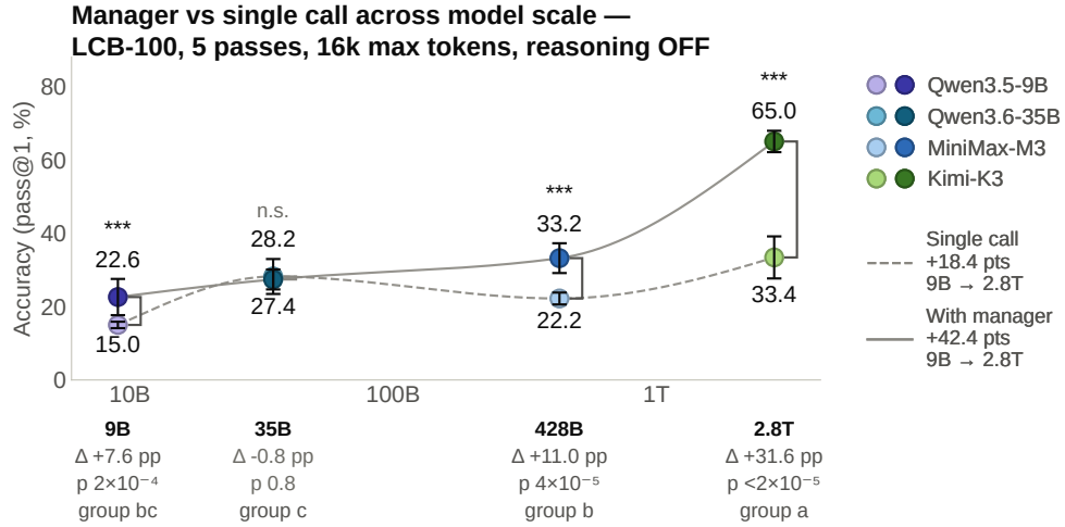
Fig. 7 Accuracy by model scale, reasoning off, 16k, five passes. The same numbers as Fig. 5b, against parameter count; the line through each mark is the 95% CI across the five passes. Dashed = single call, solid = with manager, and the bracket at a pair grades its Holm-corrected p; the block under each tick gives that model's \Delta , p and Tukey group, and the legend each arm's gain from 9B to 2.8T.
