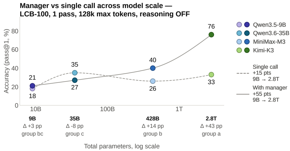
Fig. 8 Accuracy by model scale, reasoning off, 128k, one-pass control. The same numbers as Fig. 5c, against parameter count. Dashed = single call, solid = with manager; the block under each tick gives that model's \Delta and Tukey group, and the legend each arm's gain from the smallest model to the largest.
