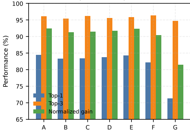
(b) Optimal-beam prediction
