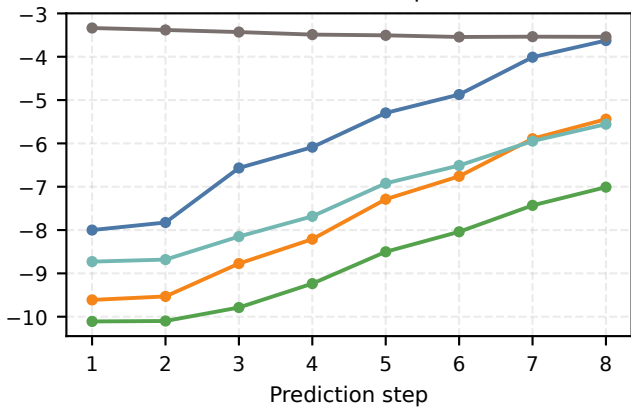
(a) Recursive full-CSI prediction
