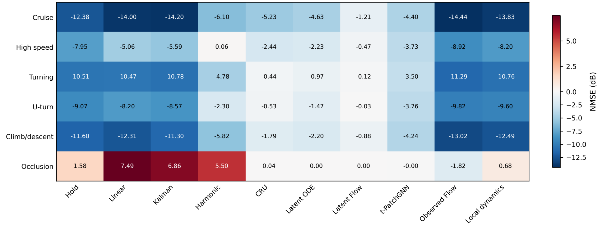
Full-matrix per-target NMSE (dB); lower is better
