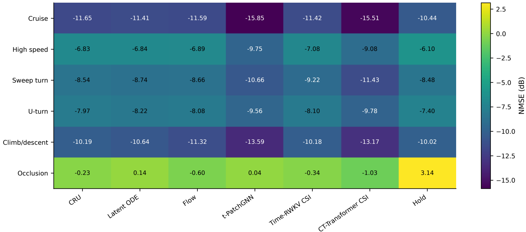
Independent ray-traced off-grid queries: NMSE (dB)
