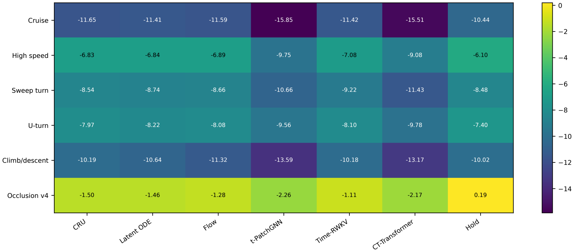
Independent ray-traced off-grid NMSE (dB)
