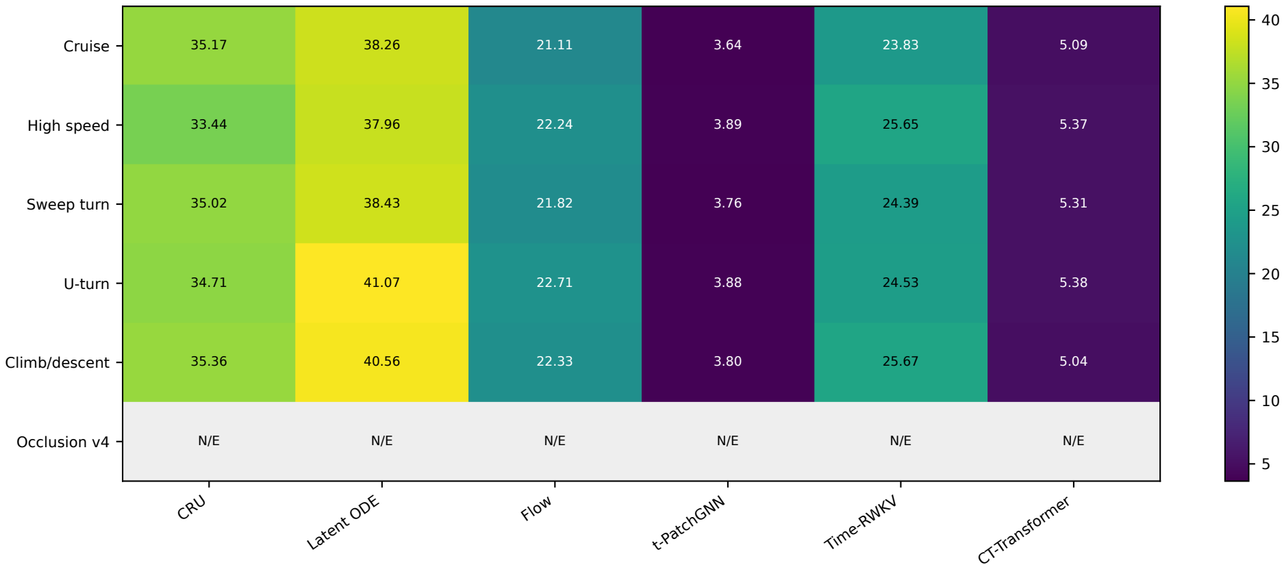
Batch-1 full-CSI latency (ms); v4 not measured (N/E)
