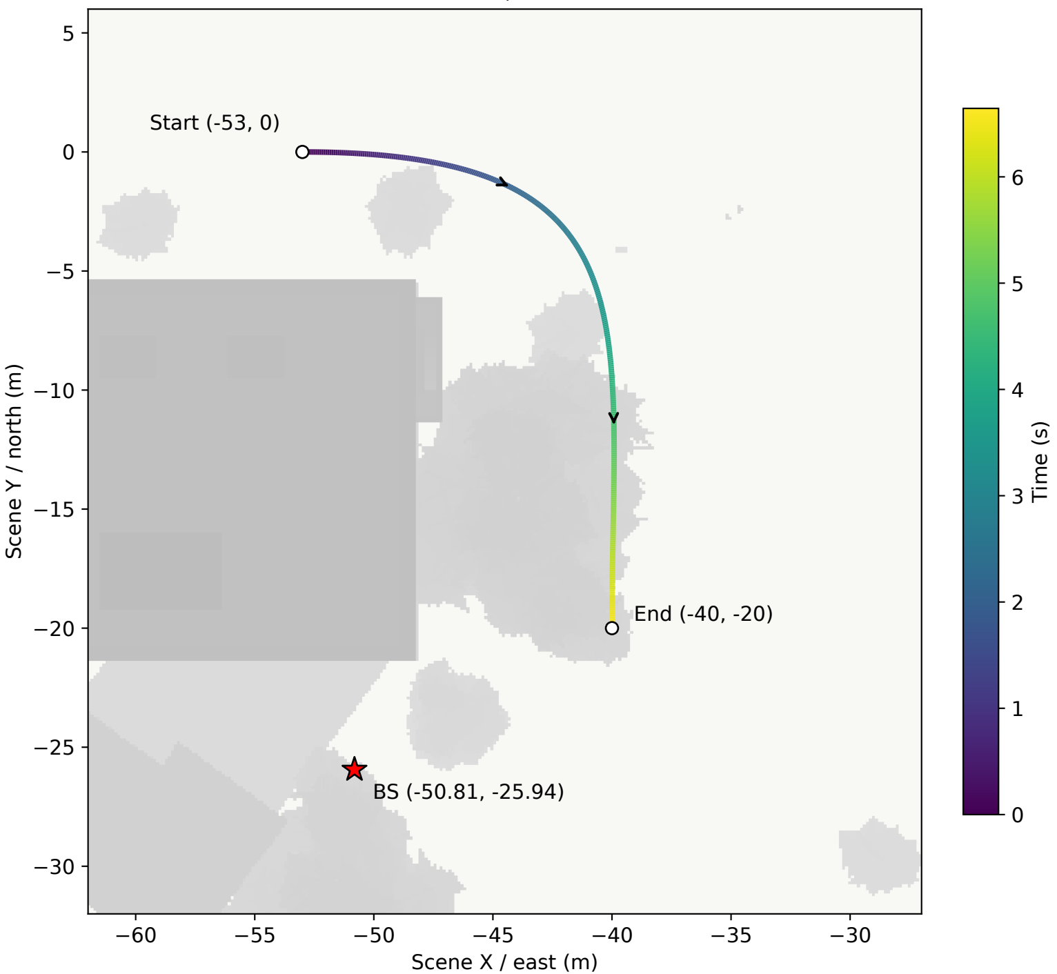
site_03: curved route UAV z=20.62 m; BS z=24.37 m
