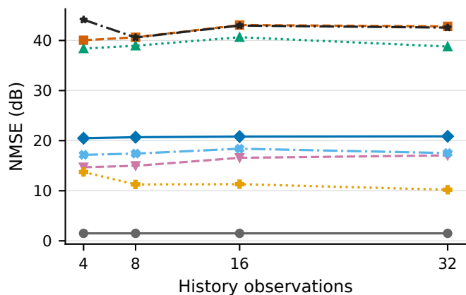
Dropout
