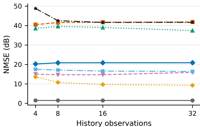
Bursty
