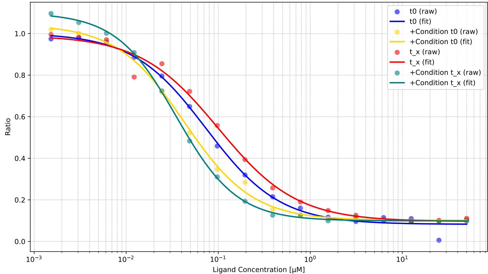
Binding Affinity Curves for X1
