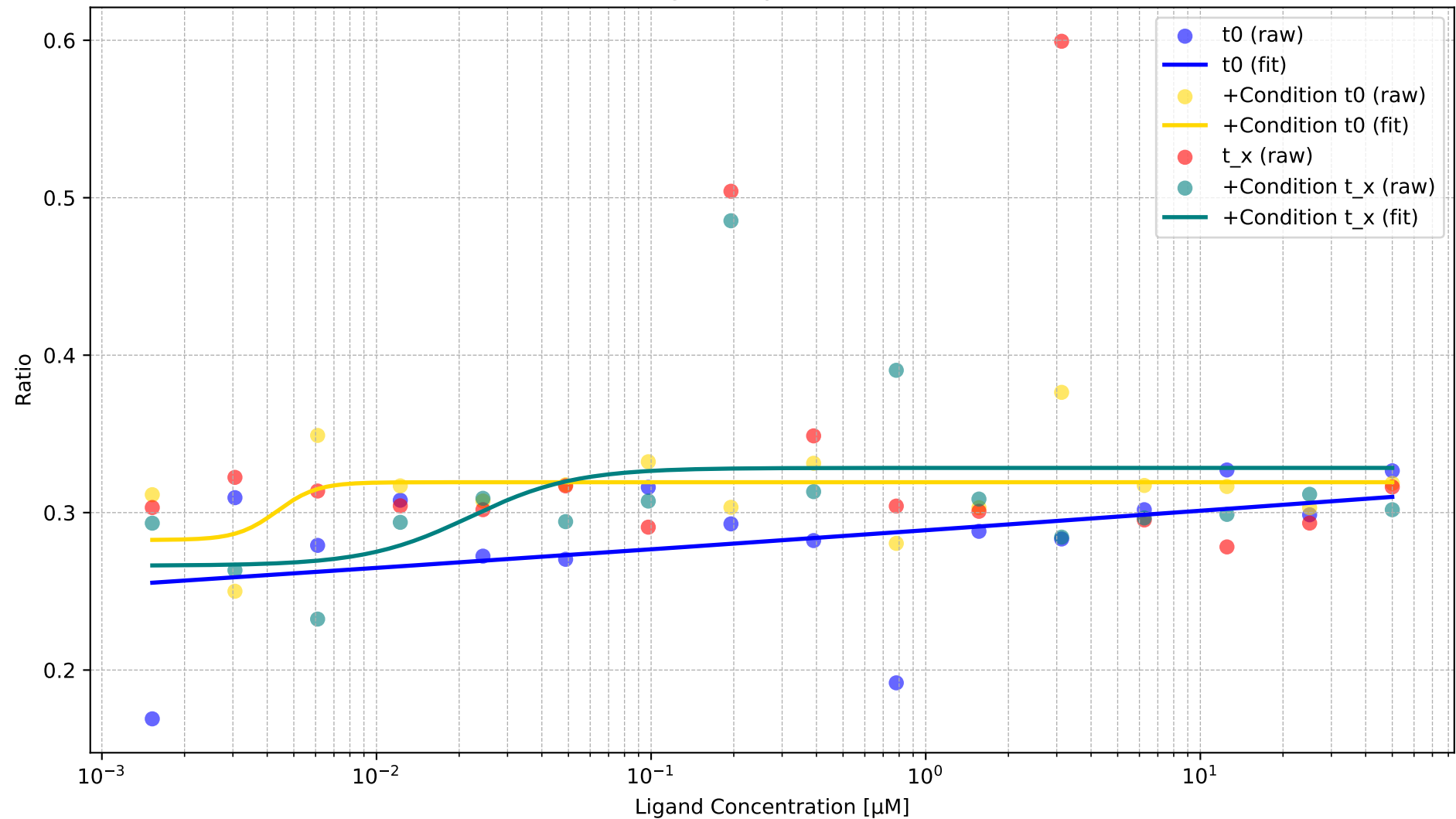
Binding Affinity Curves for X7
