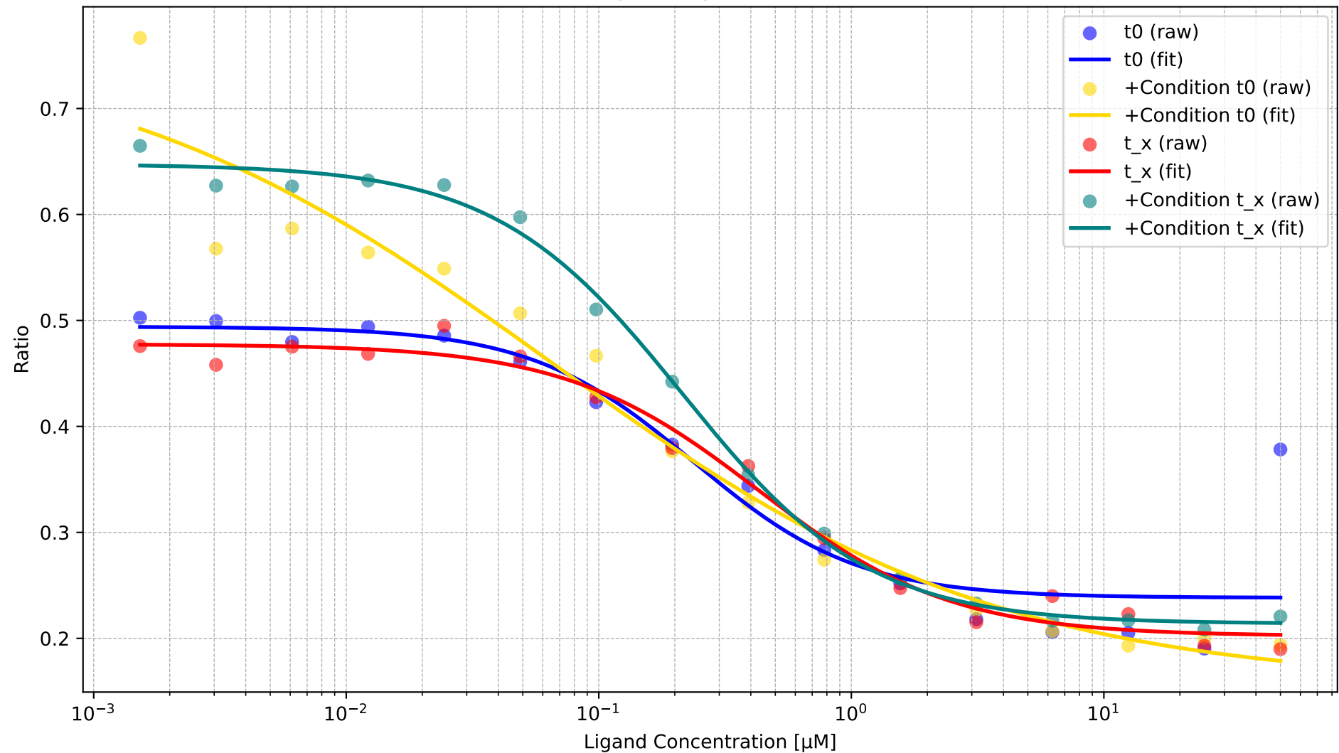
Binding Affinity Curves for X4
