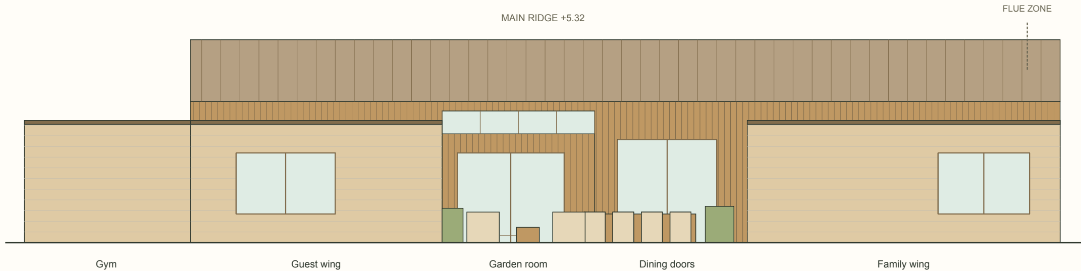
A / FROM THE MAIN GARDEN: GYM LEFT, FAMILY WING RIGHT
