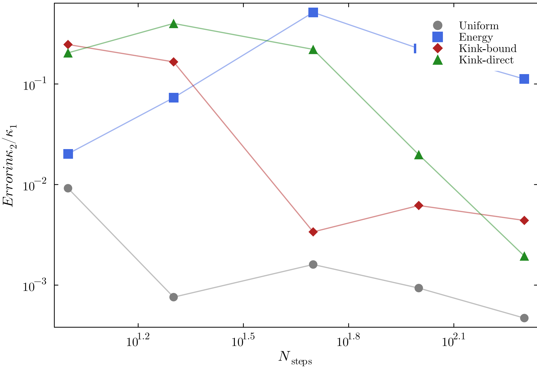
Cumulant ratio error ( L = 20, \tau_Q = 10.0 )
