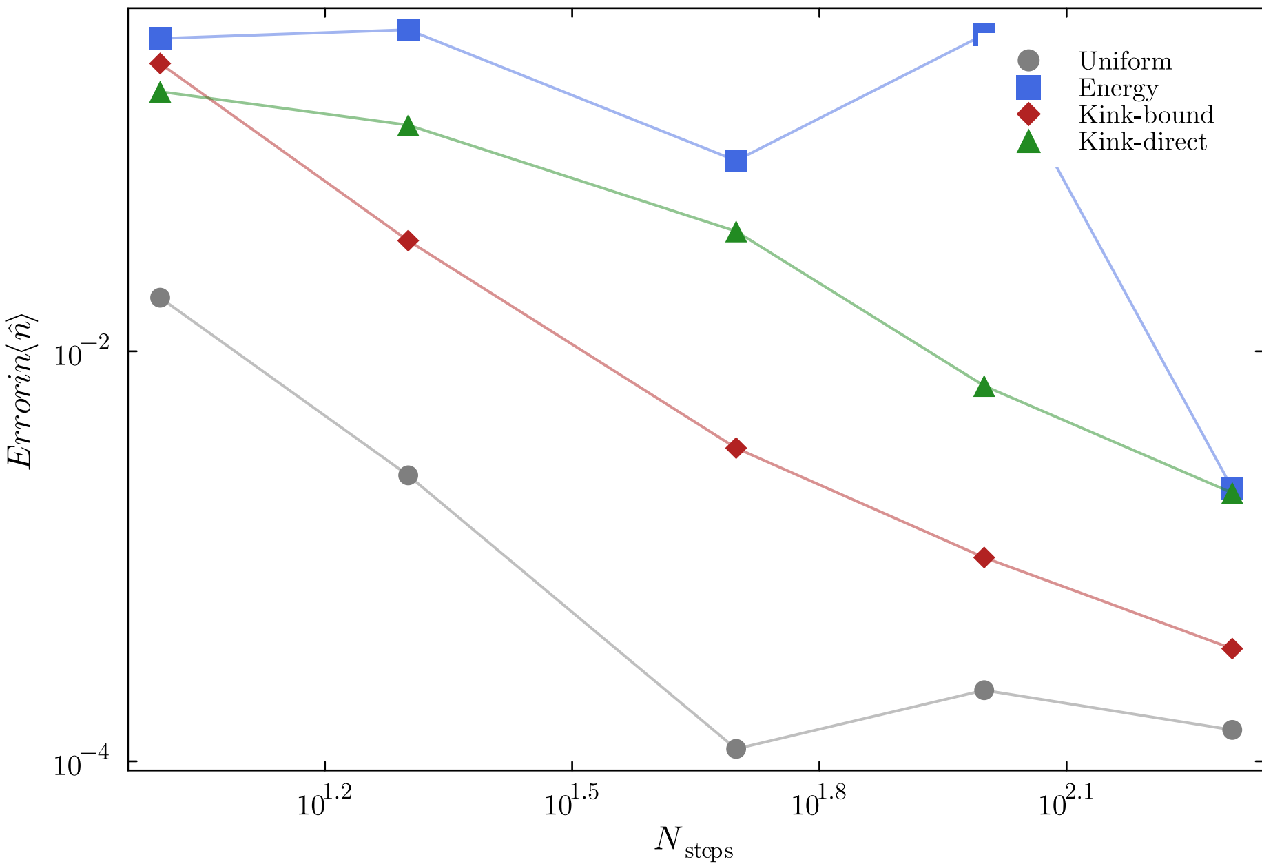
Kink density error ( L = 20, \tau_Q = 10.0 )
