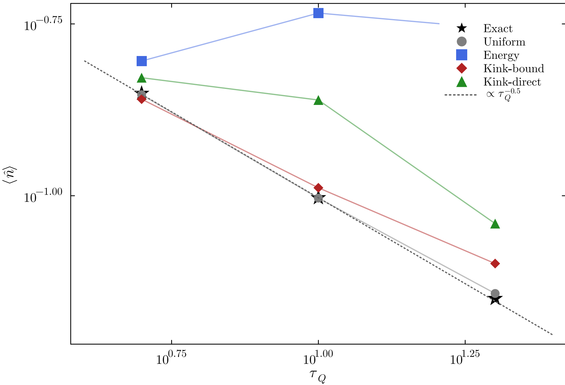
KZM scaling with N = 50 Trotter steps
