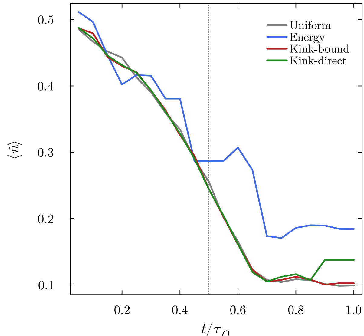
\langle \hat{n} \rangle(t) trajectories
