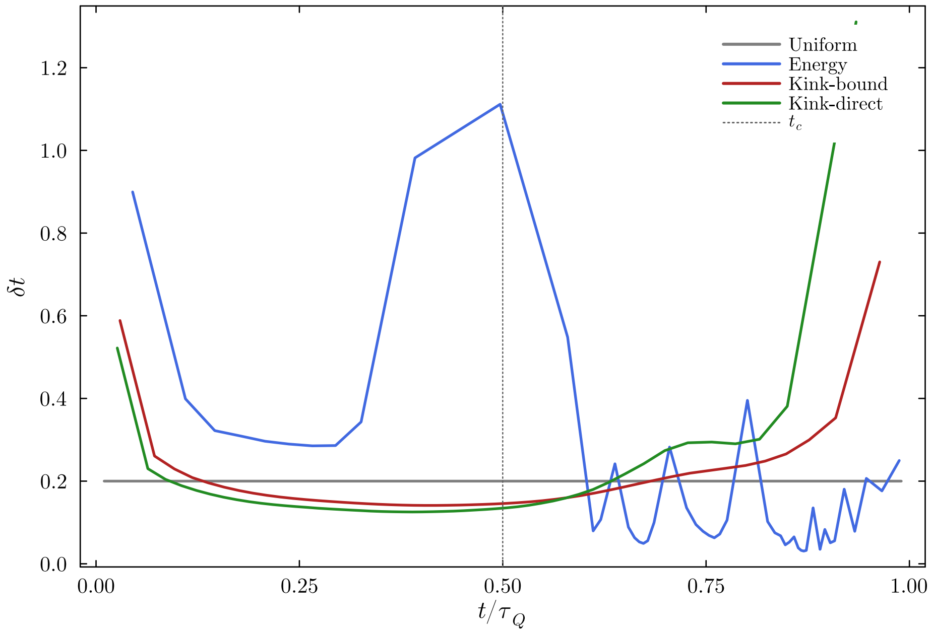
Step sizes for N = 50 , \tau_Q = 10.0
