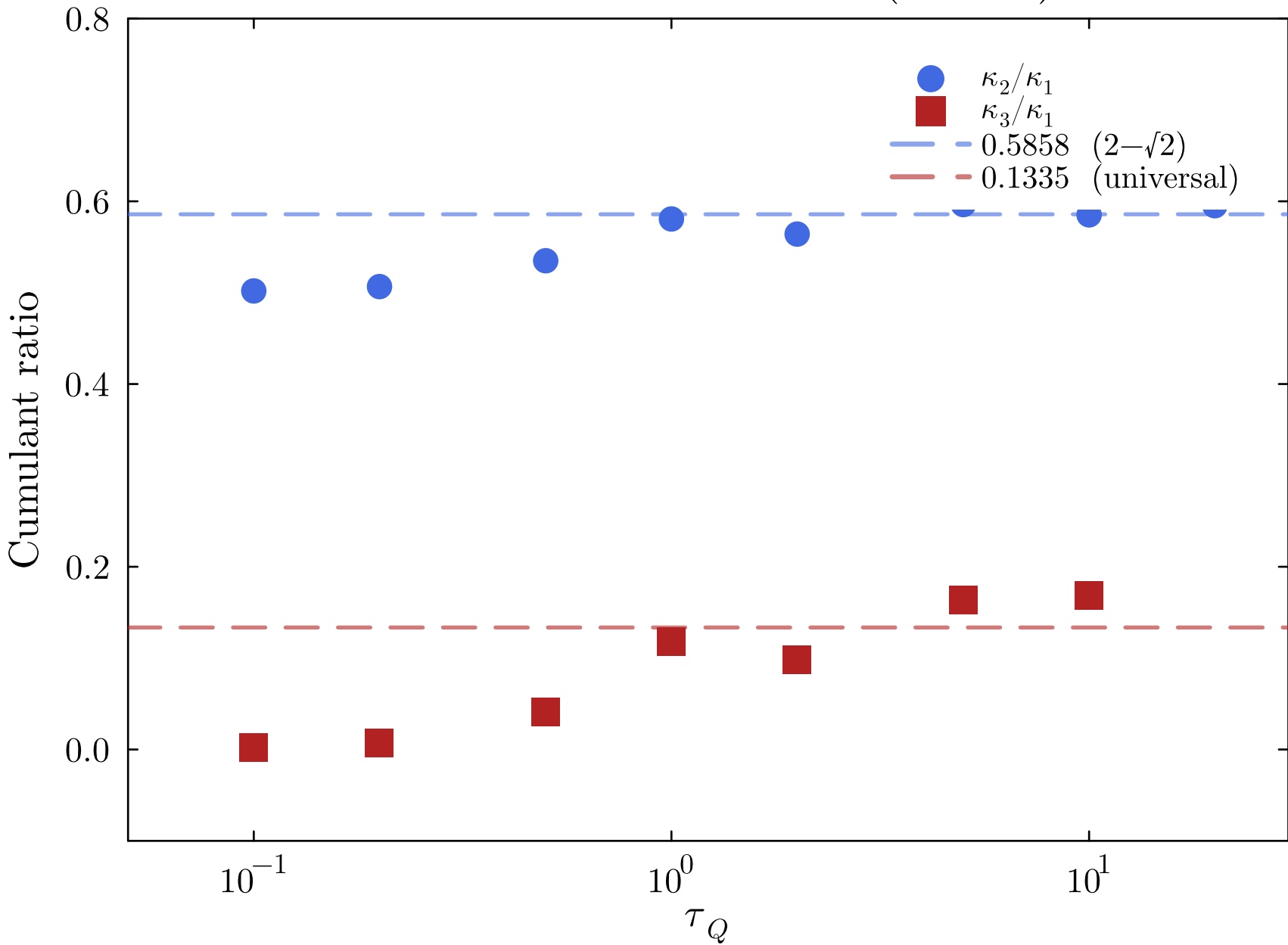
Universal cumulant ratios ( L = 100 )
