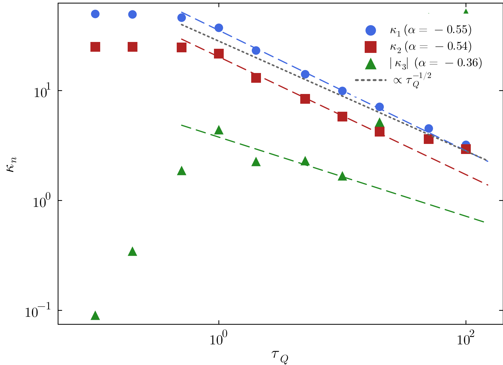
Kink number cumulants ( L = 100 )
