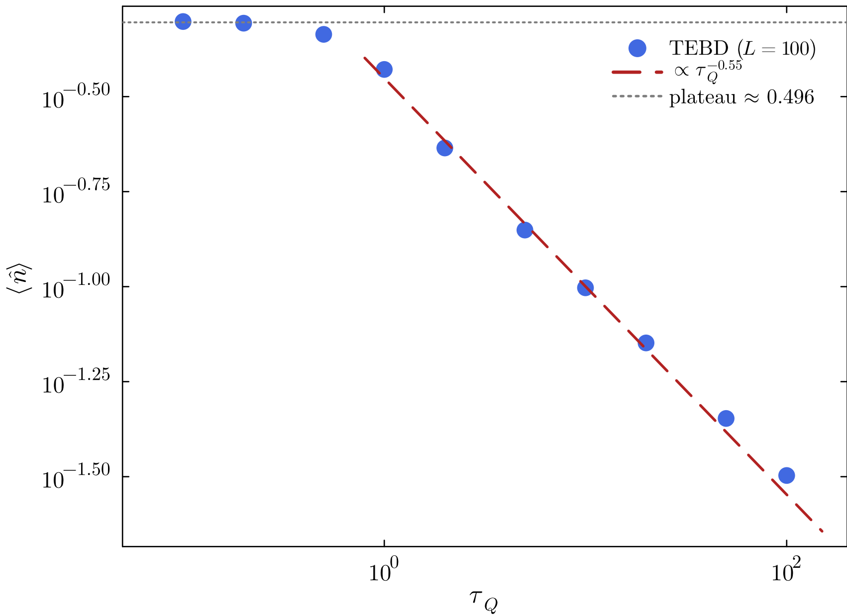
Kink density ( L = 100 )
