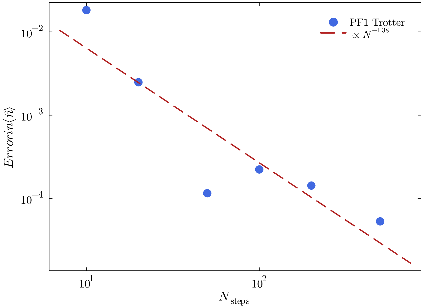
Trotter error in kink density ( L = 20, \tau_Q = 10.0 )
