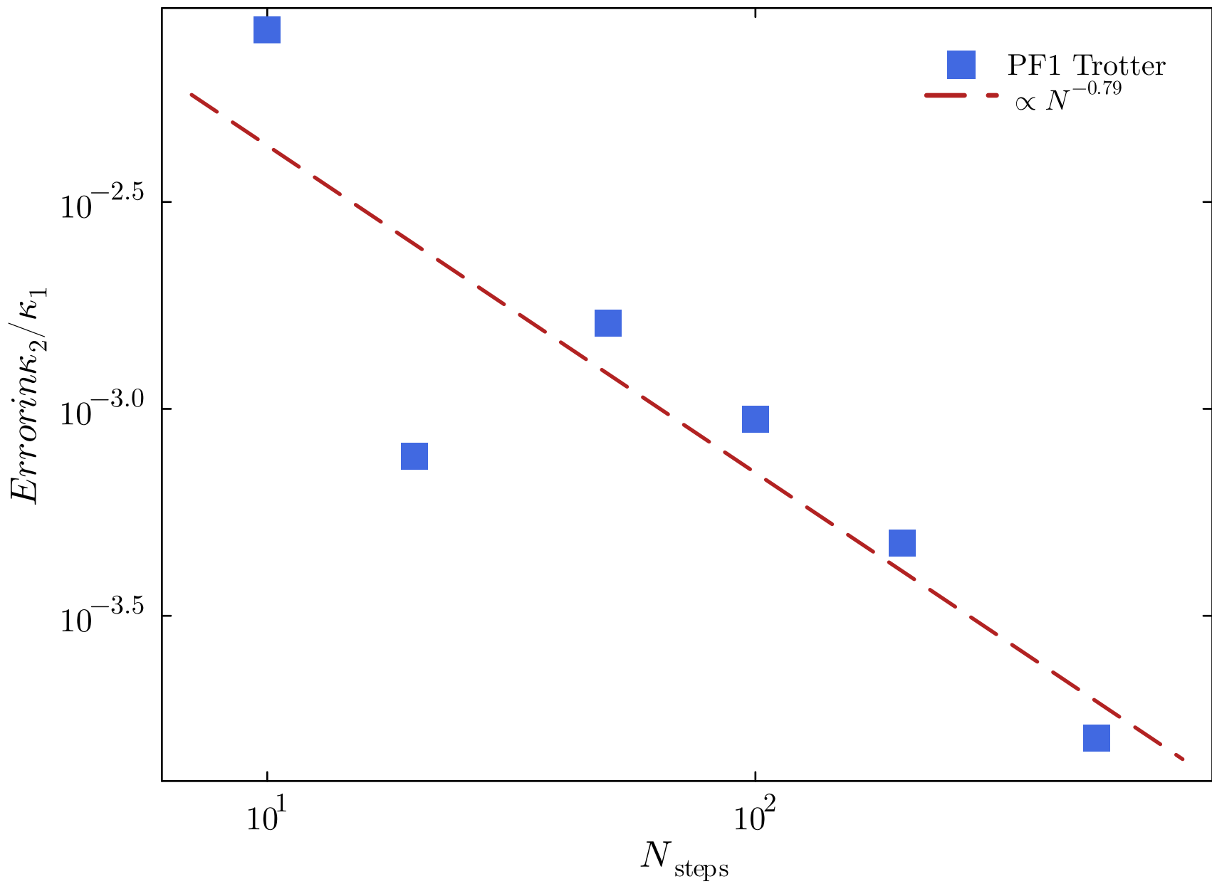
Trotter error in cumulant ratio ( L = 20, \tau_Q = 10.0 )
