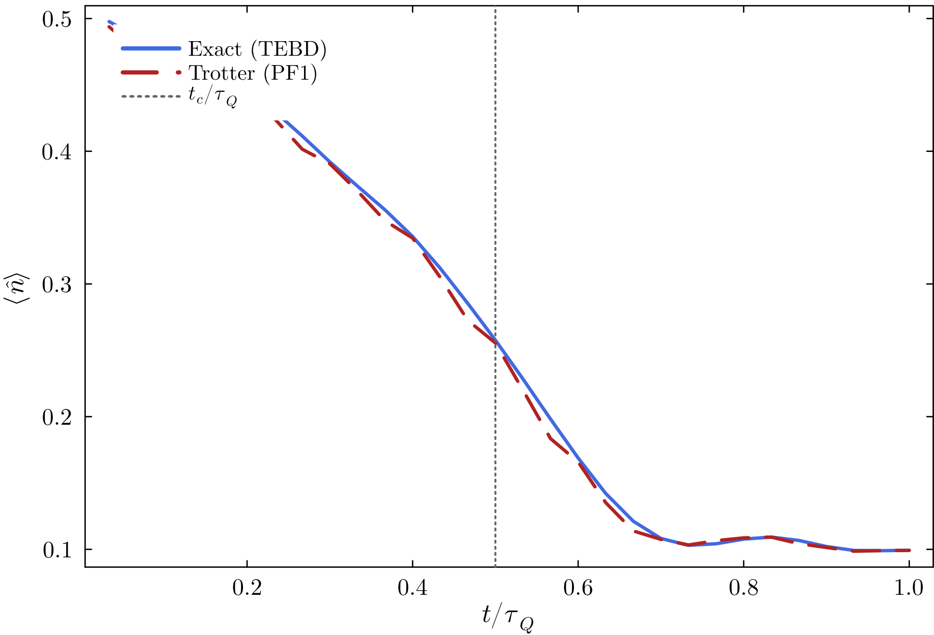
Kink density: exact vs Trotter ( N = 50 )
