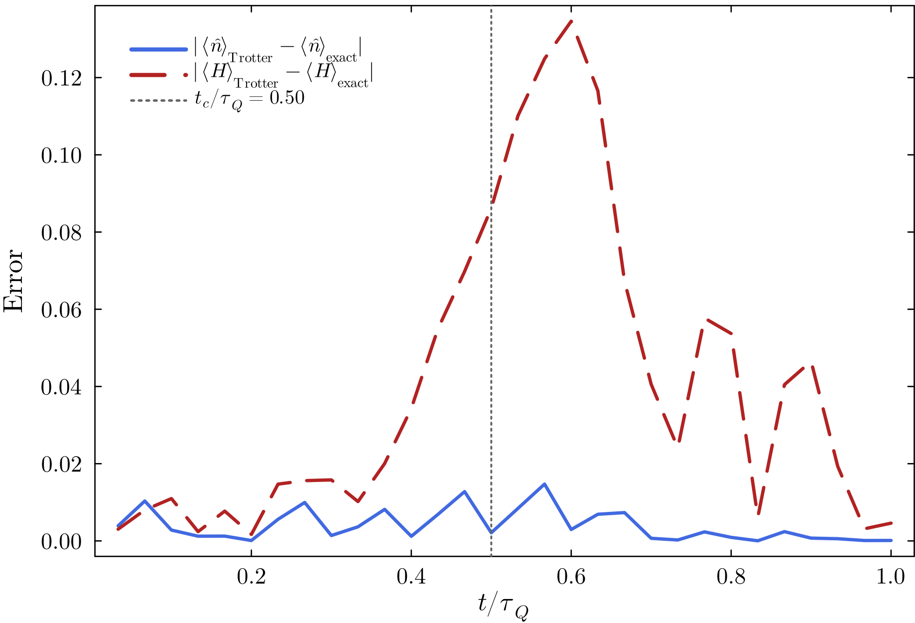
Time-resolved Trotter errors ( N = 50 )
