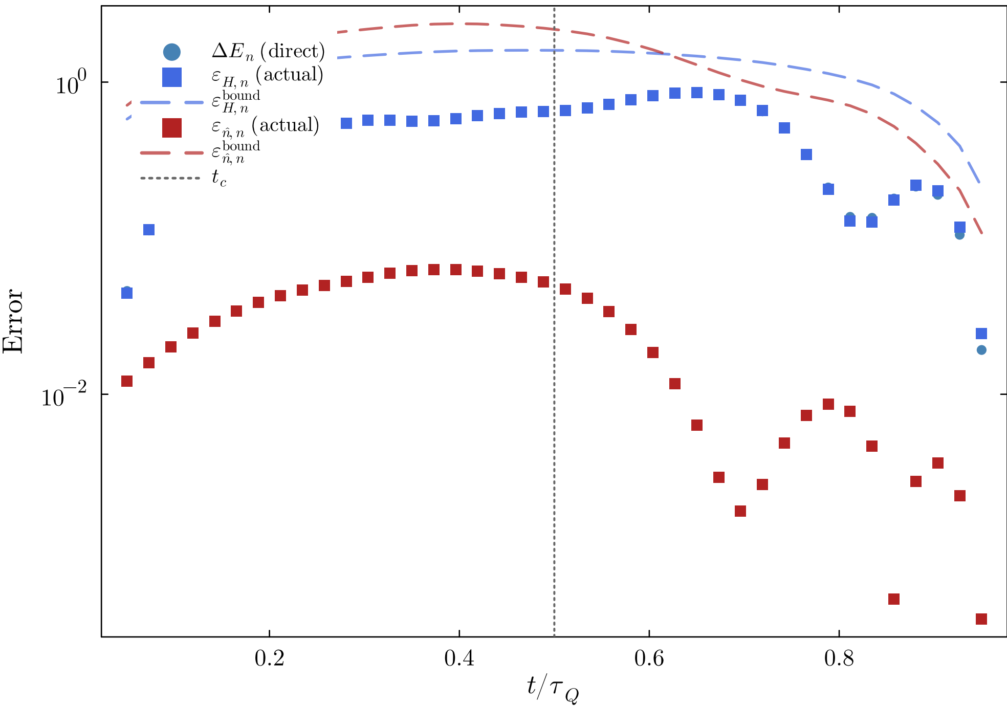
Verification hierarchy ( L = 20, \delta t = 0.5 )
