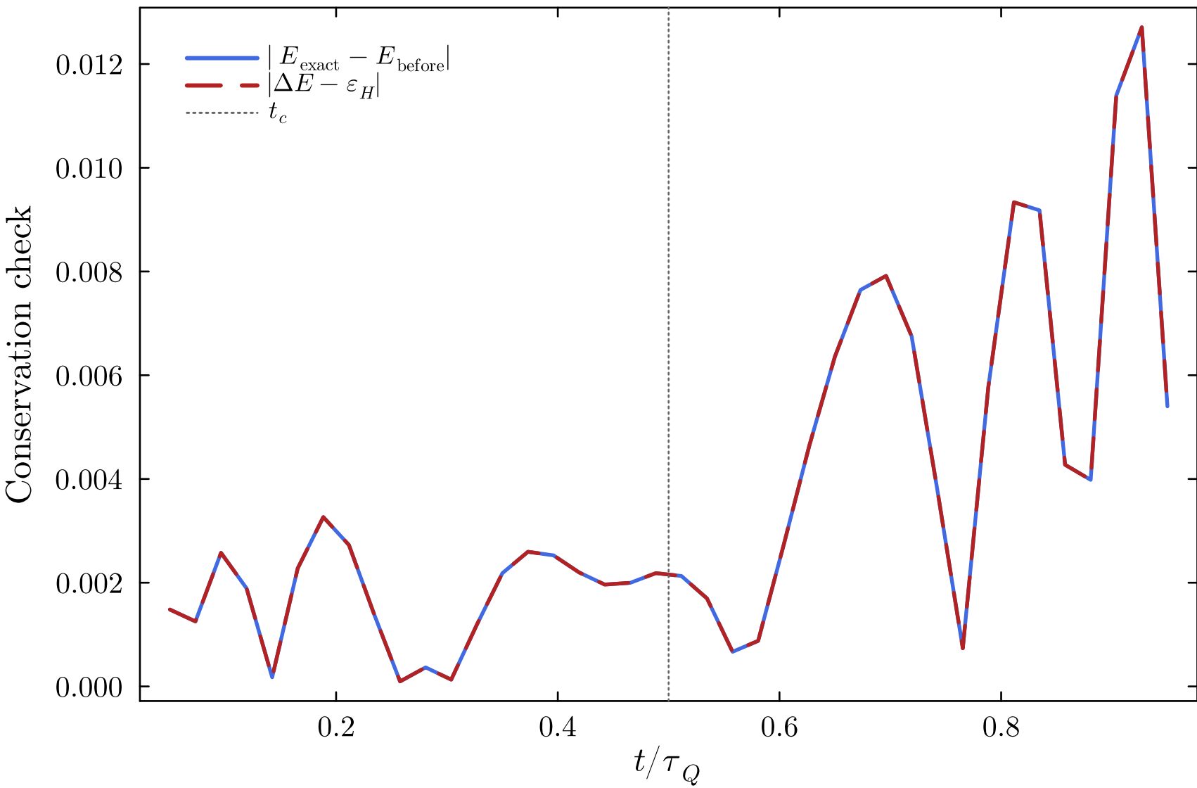
Piecewise conservation (200 substeps, L = 20 )
