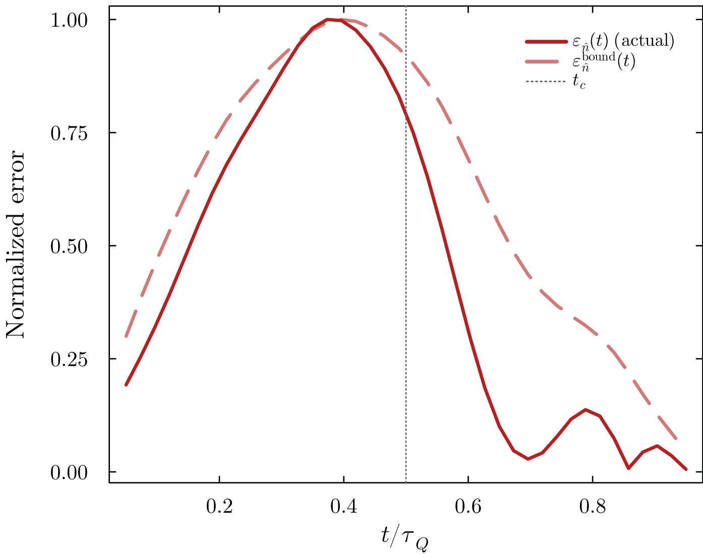
Kinkdensity (corr = 0.936)
