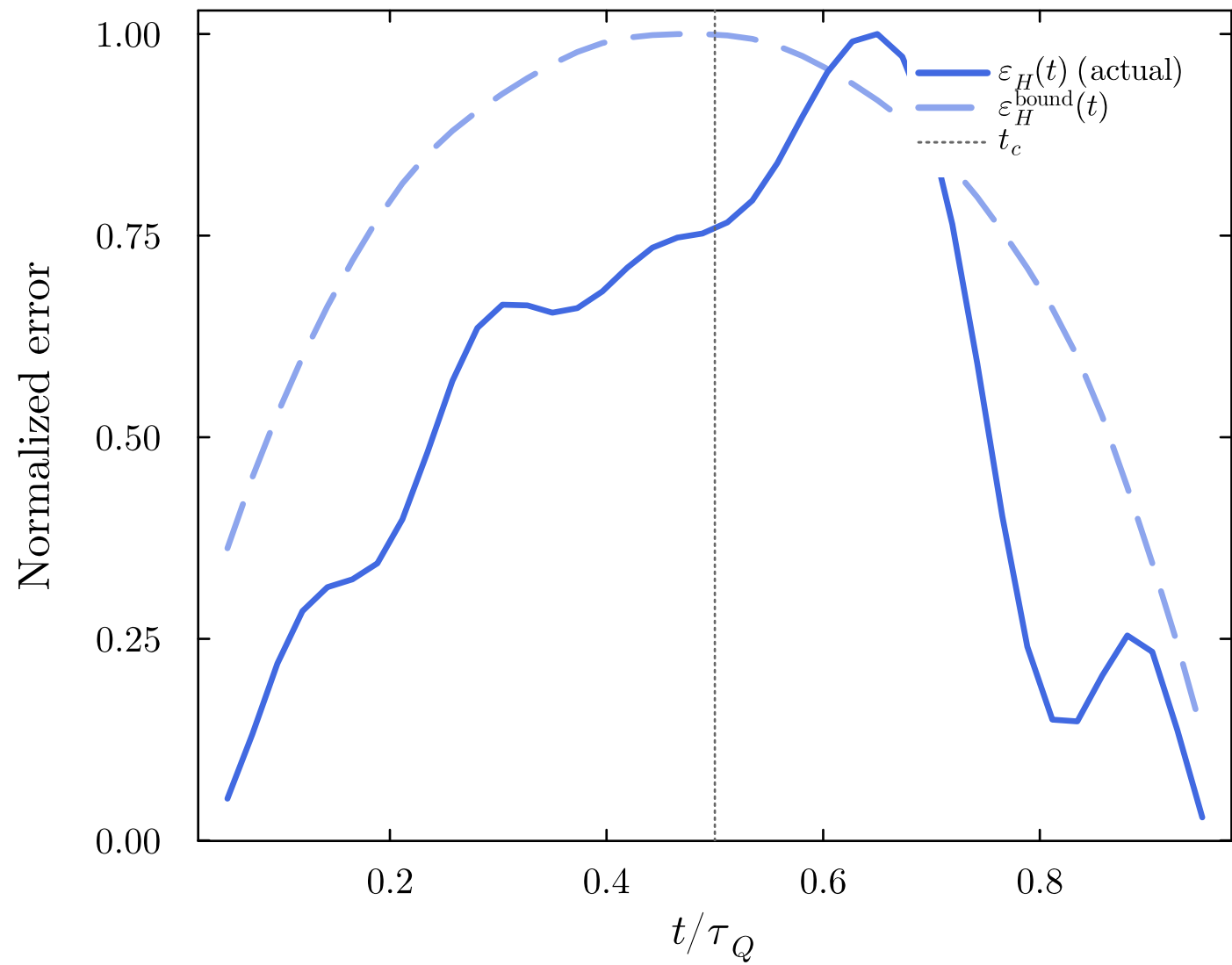
Energy (corr = 0.859)
