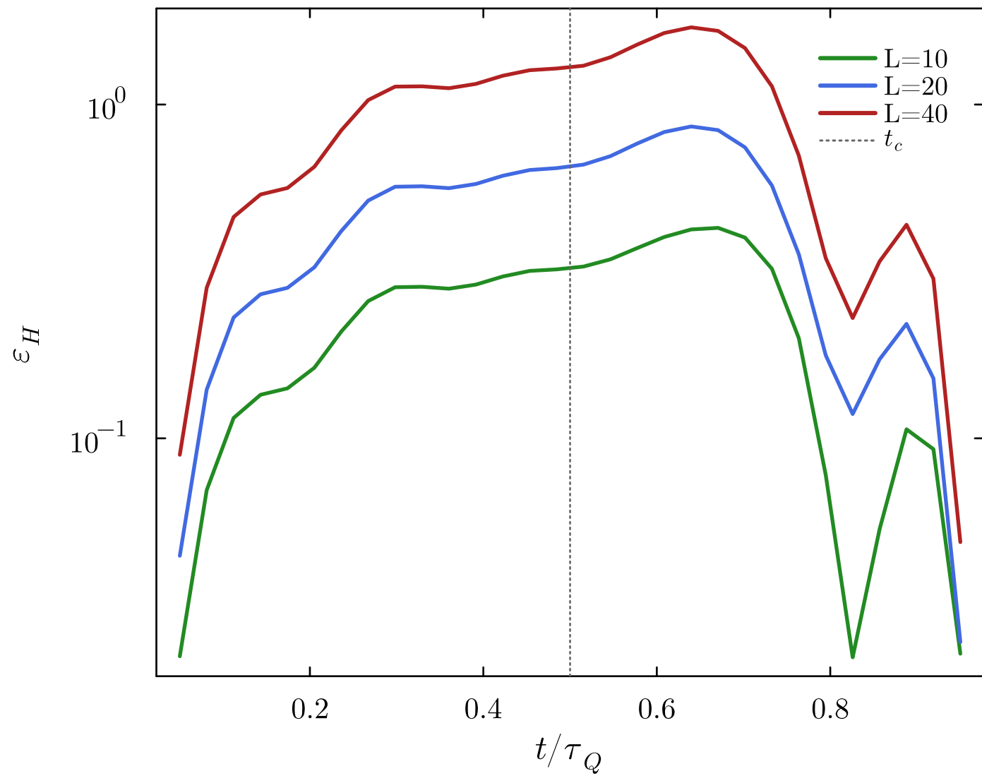
Energy Trotter error
