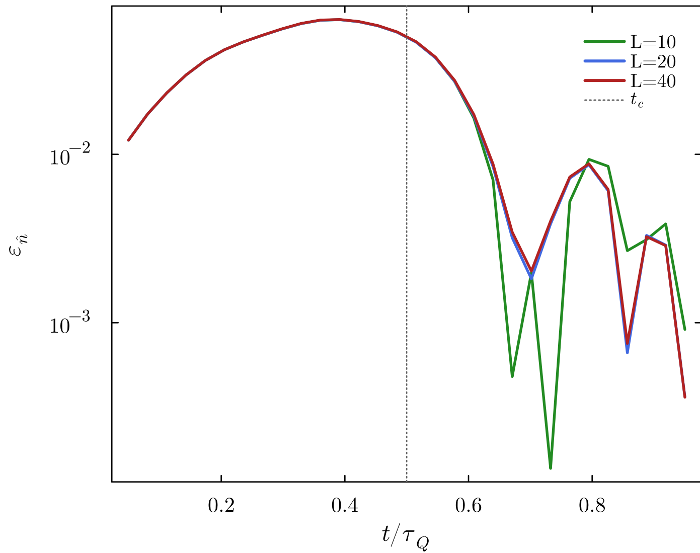
Kink density Trotter error
