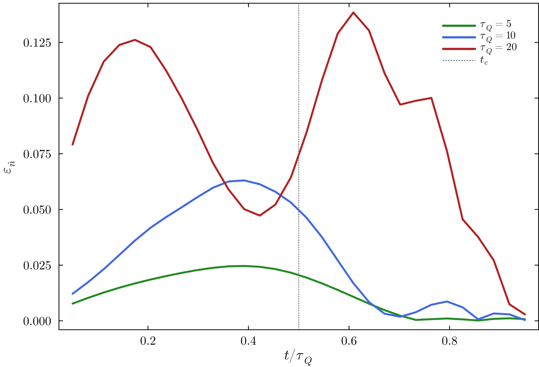
Kink density error: \tau_Q dependence ( L = 20 )
