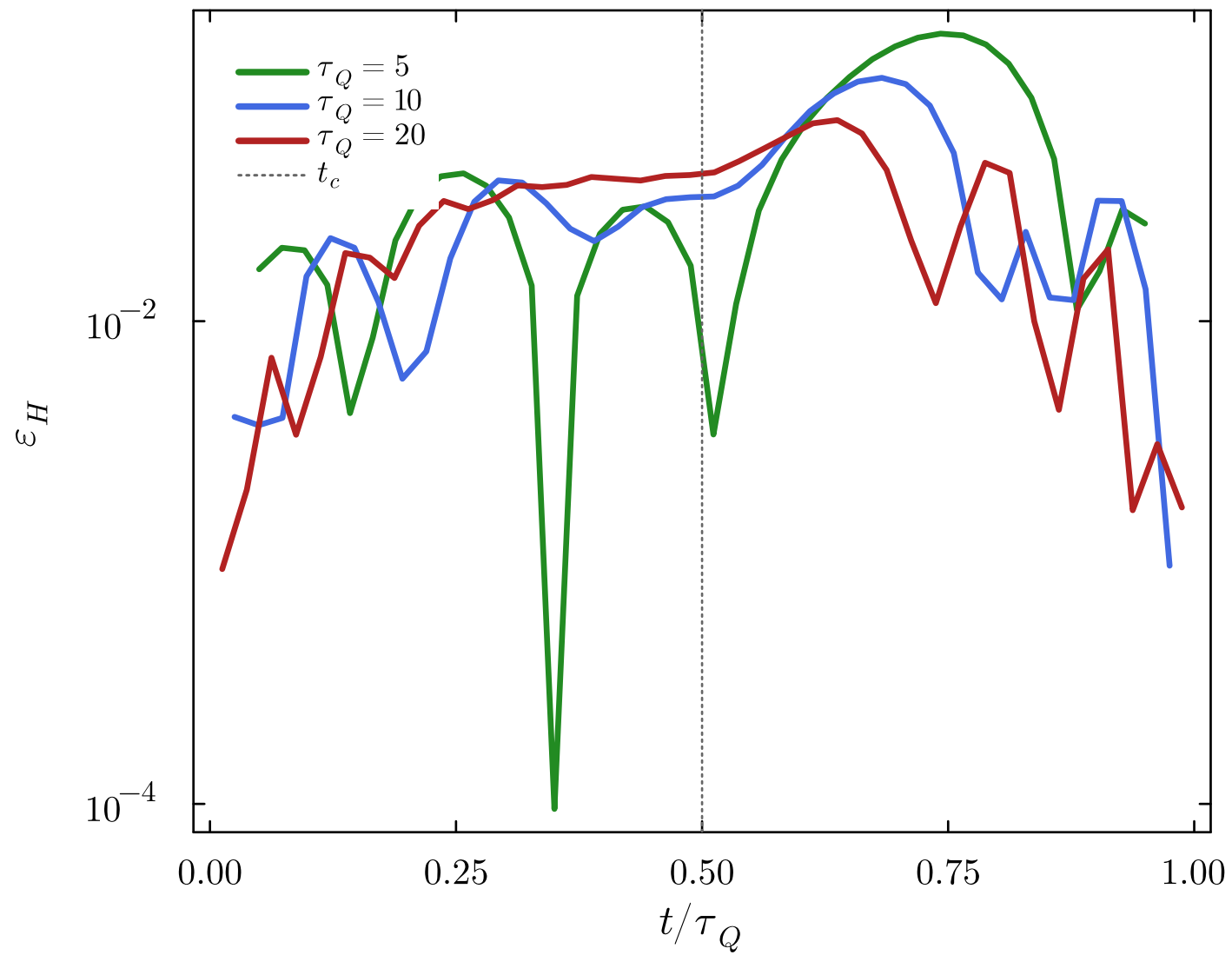
Energyerror ( \delta t = 0.25 )
