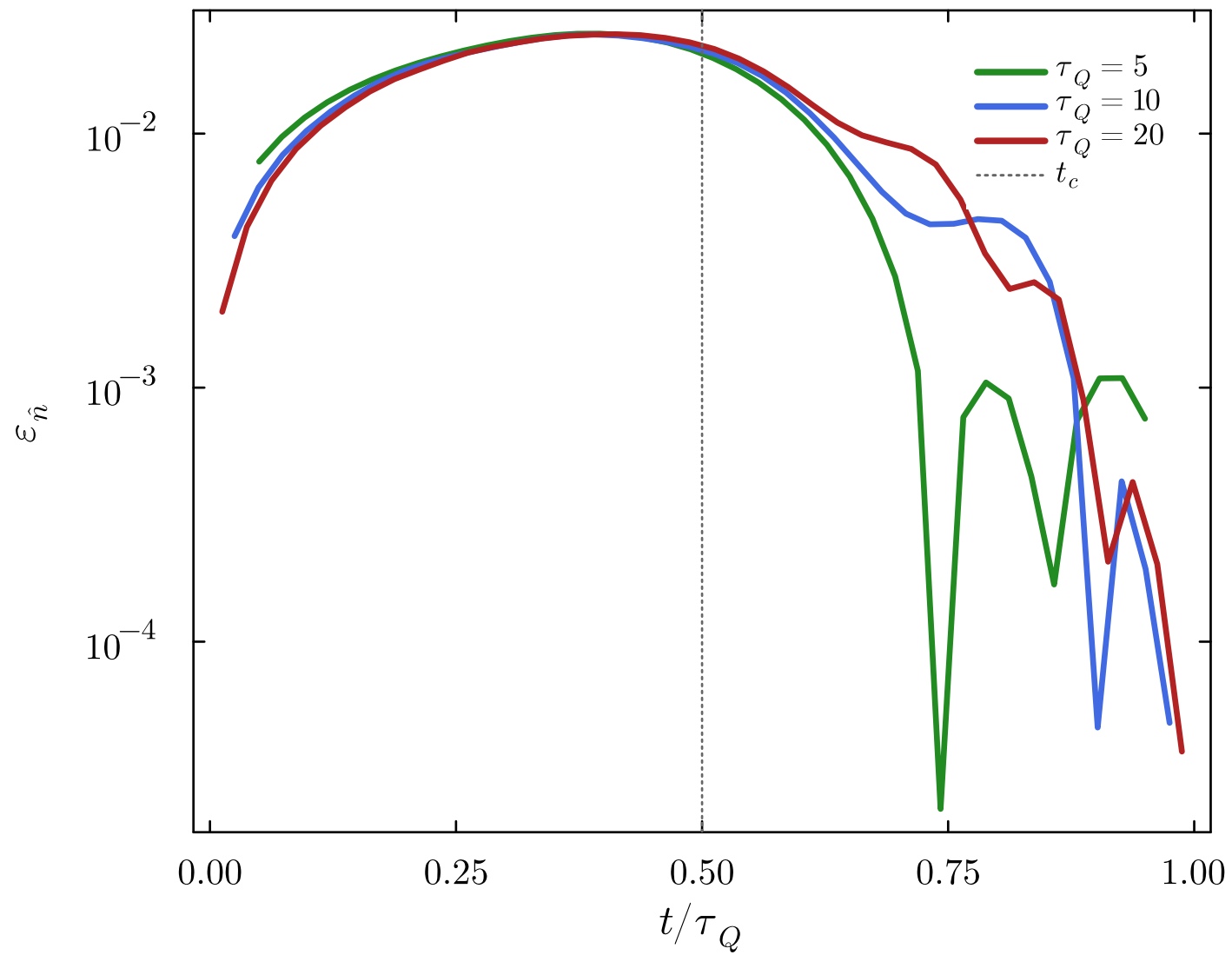
Kinkdensityerror ( \delta t = 0.25 )
