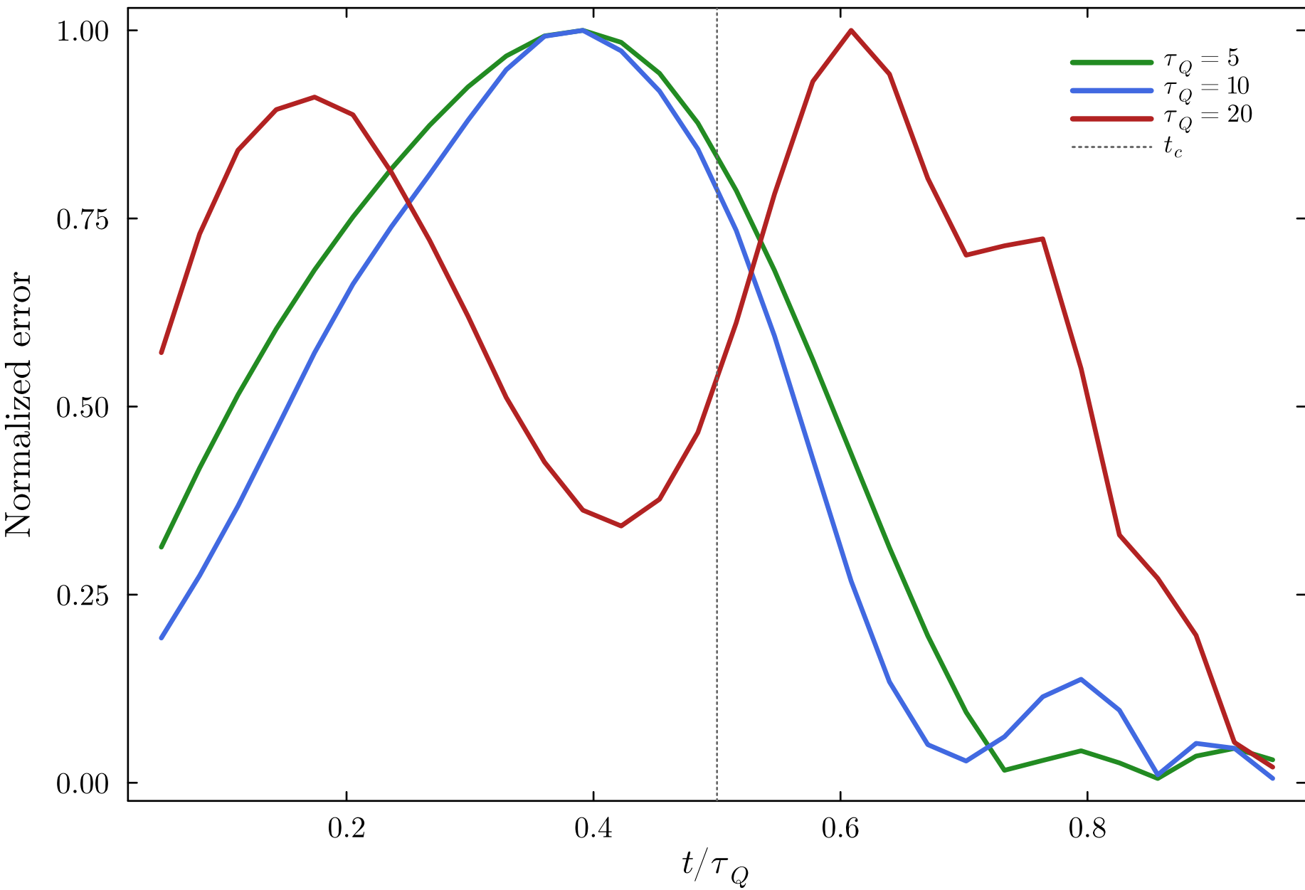
Normalized \epsilon_{\hat{n}} : shape vs \tau_Q ( L = 20 )
