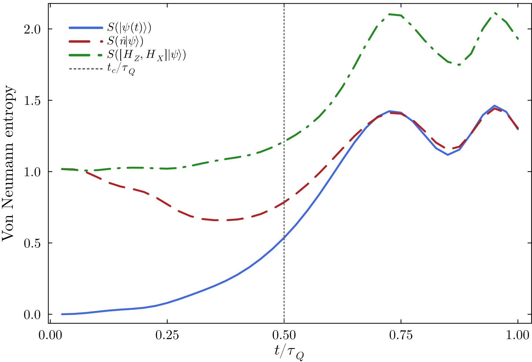
Entanglement dynamics ( L = 20 , \tau_Q = 10.0 )
