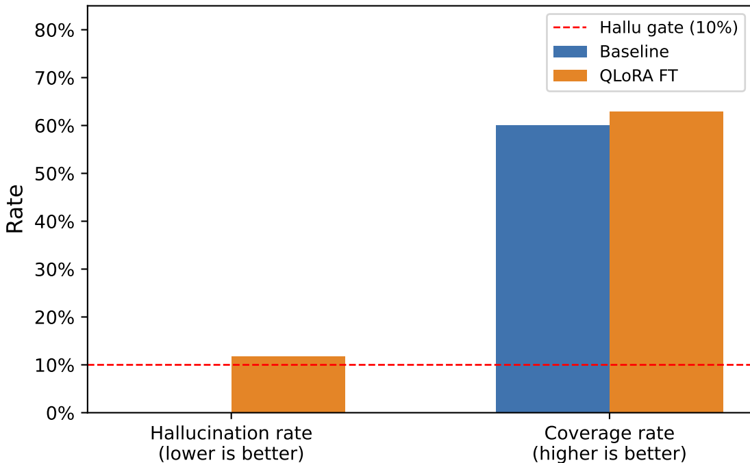
Medication Metrics: Baseline vs. QLoRA Fine-tuned
