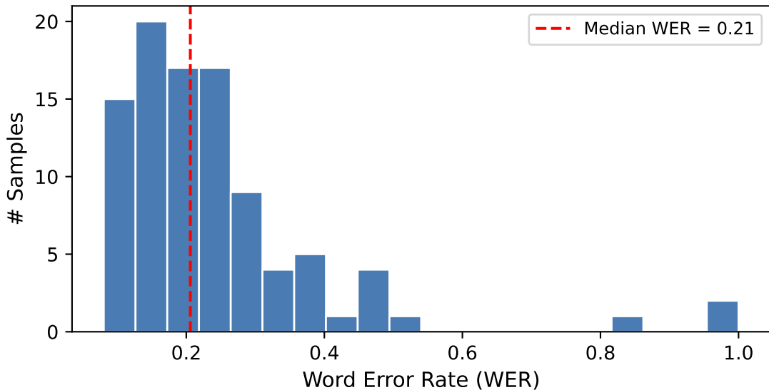
WER Distribution: whisper.cpp vs Clean Dialogue (96 val samples)
