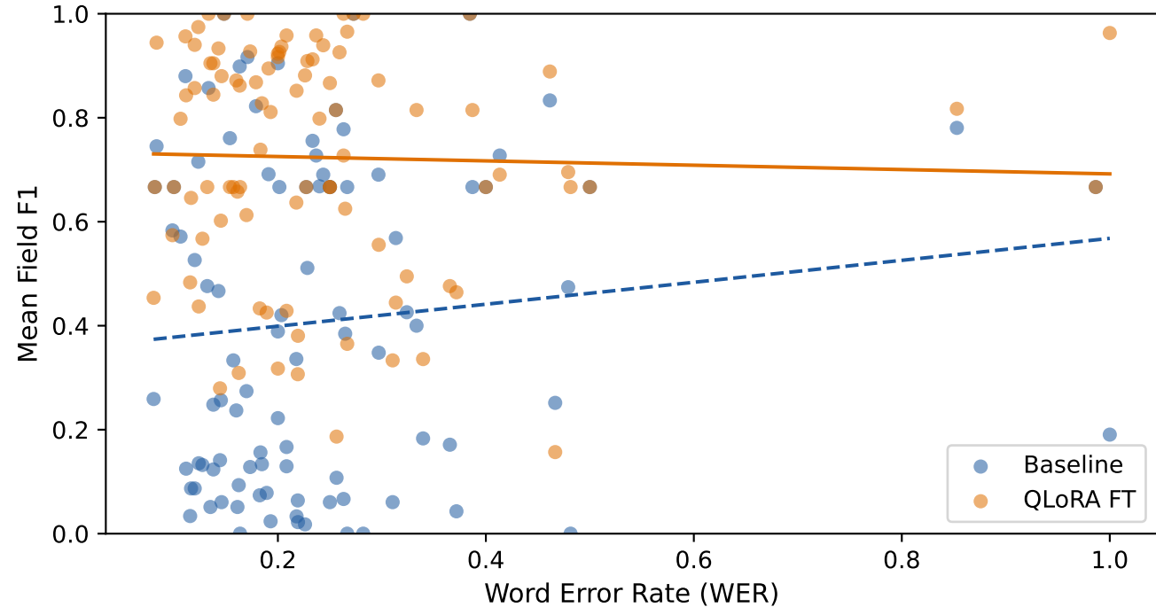
ASR Noise Robustness: WER vs. Mean Field F1
