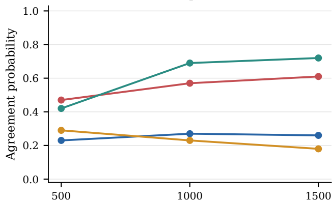
(b) BIC winner is prediction winner
