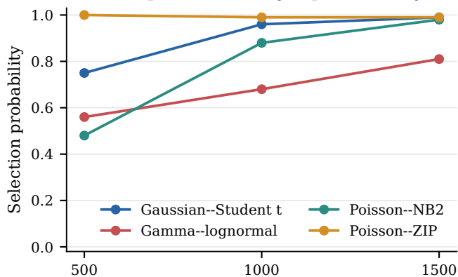
(a) Equivalent family-tuple recovery
