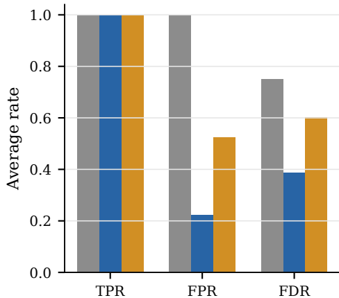
Gaussian--Student t
