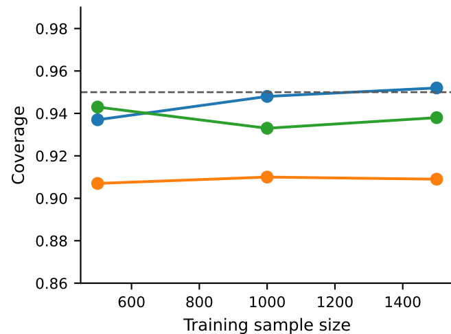
Nominal 95% intervals
