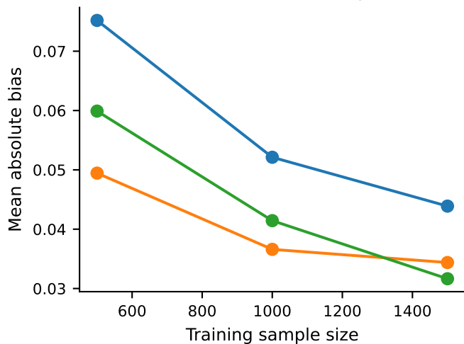
Coefficient accuracy
