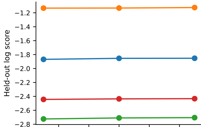
Nominal 95% intervals
