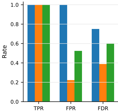
Gaussian--Student-t
