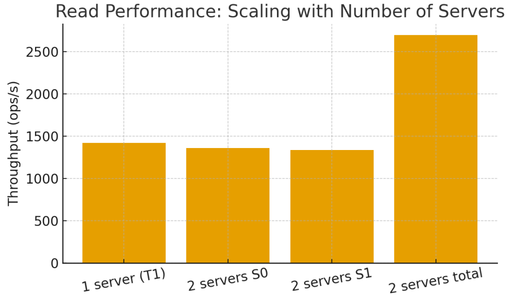
Figure 3: Read throughput scaling with two servers (sum of two concurrent clients).
