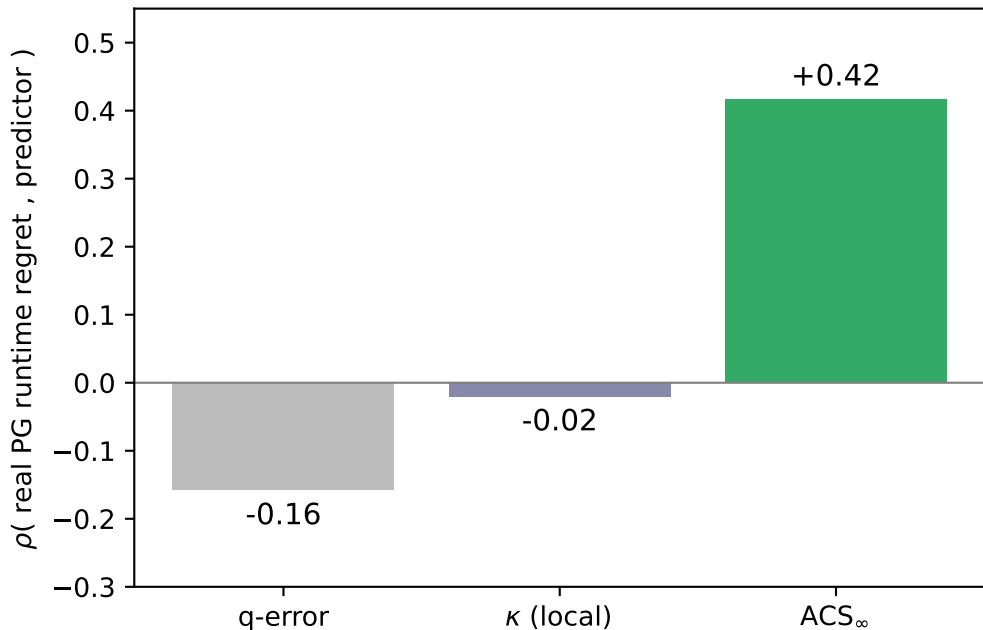
Predicting real PostgreSQL runtime regret (k=3, 110/111 queries; injected estimator cardinalities)
