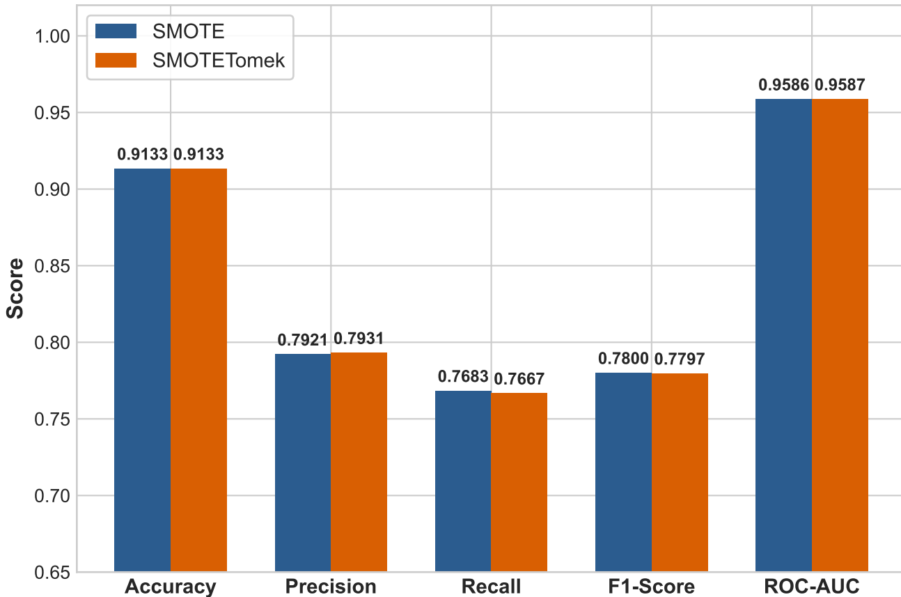
Model Performance Metrics (Accuracy, Precision, Recall, F1, ROC-AUC)
