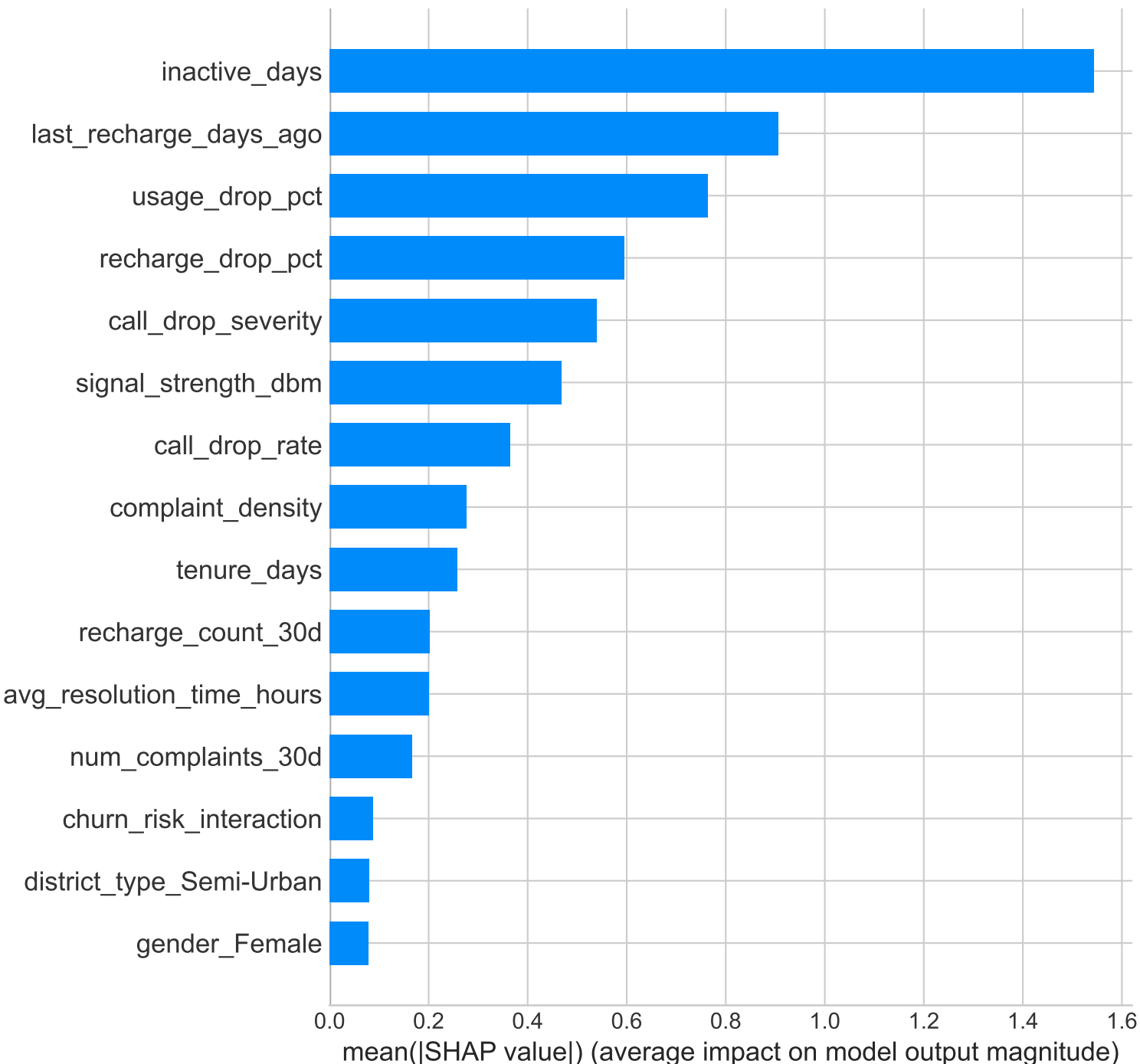
Global Feature Importance (Mean |SHAP Value|)
