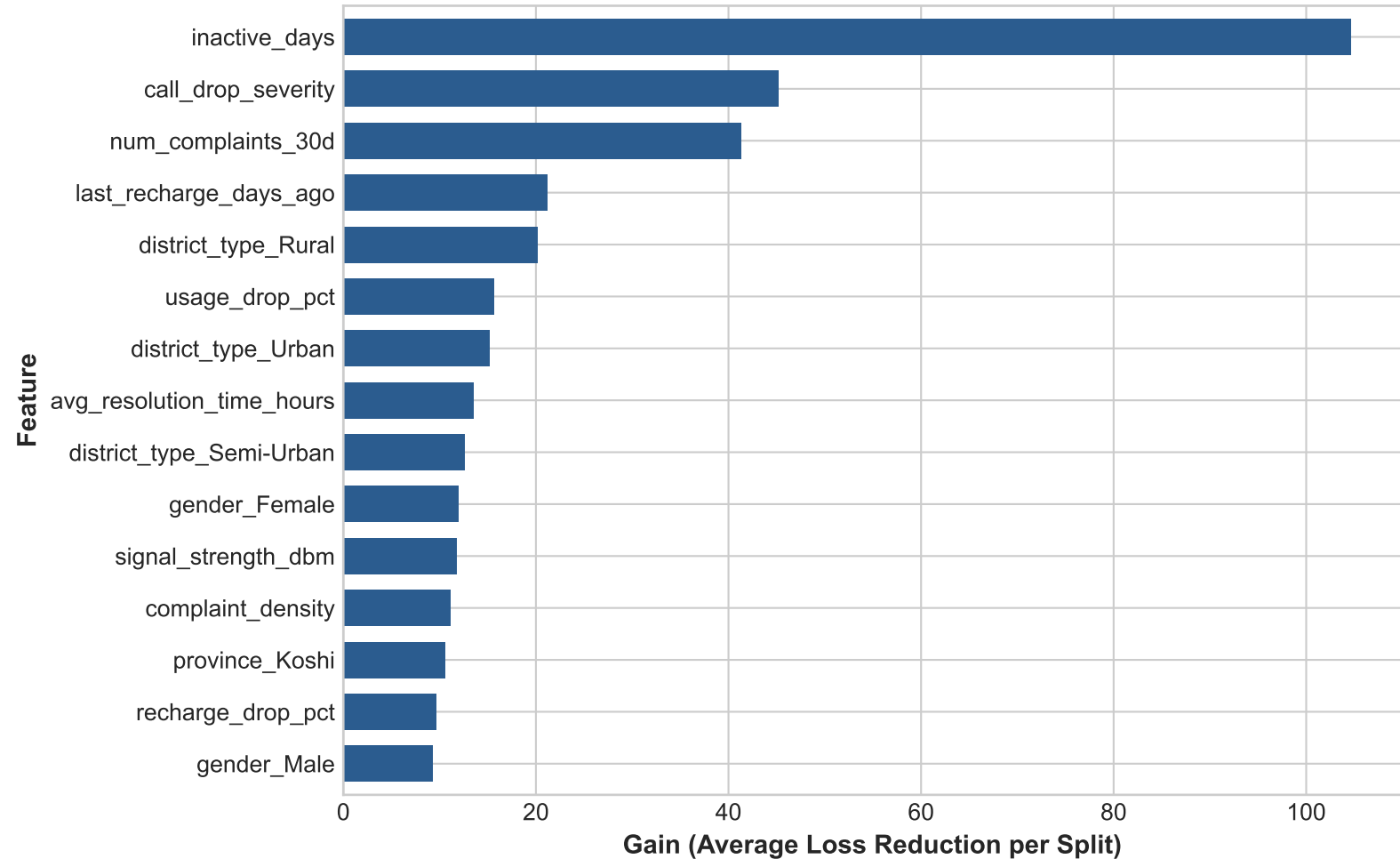
Top 15 XGBoost Feature Importances (Gain)
