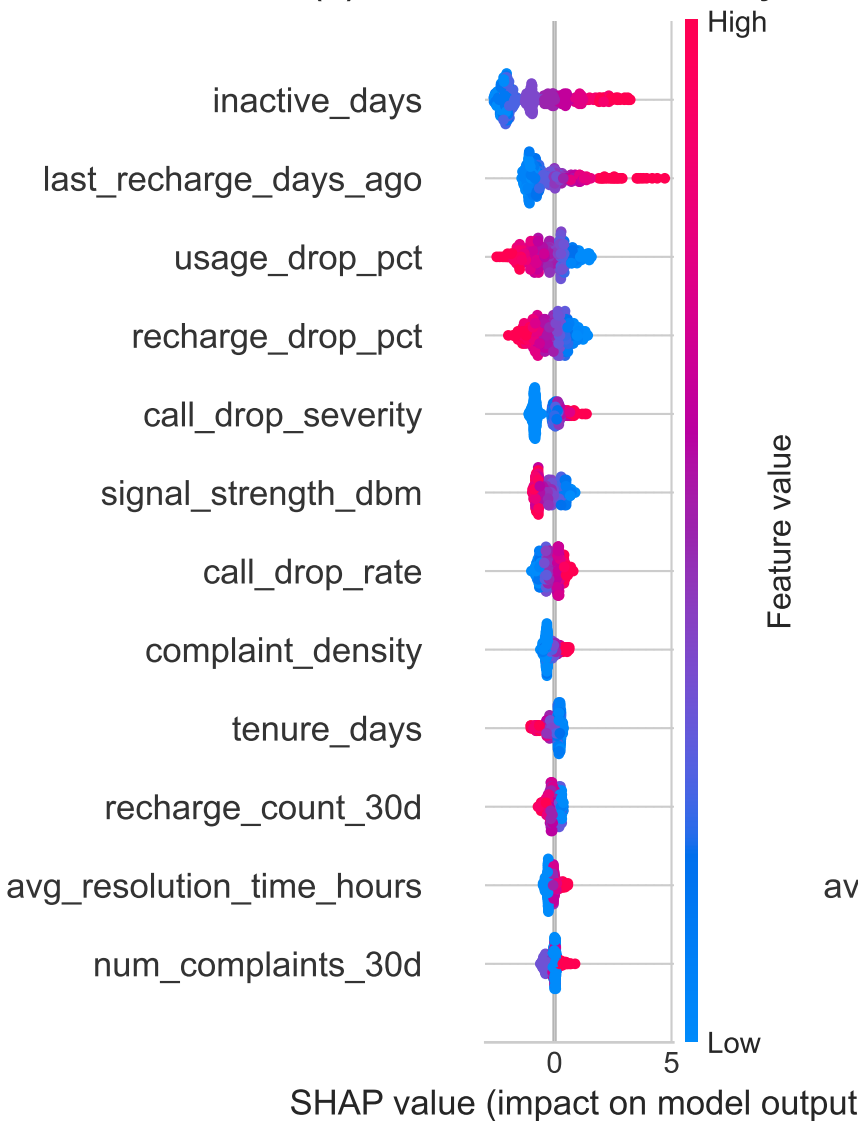
(A) SHAP Beeswarm Summary Plot
