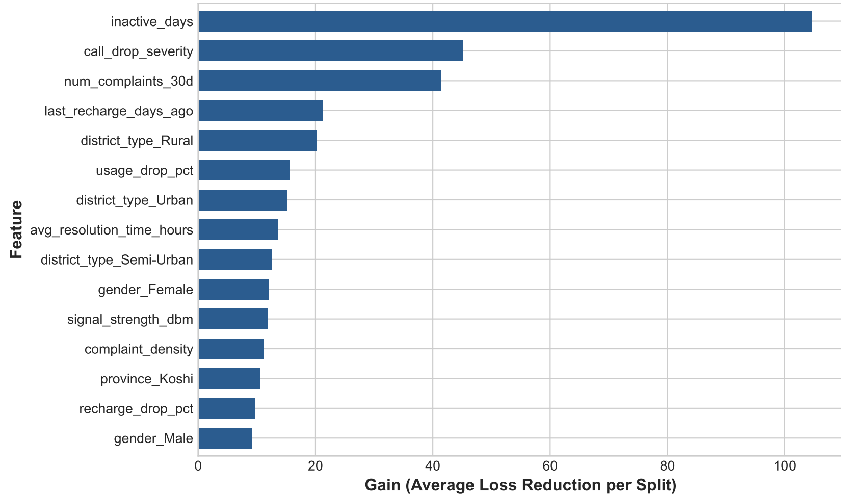
Top 15 XGBoost Feature Importances (Gain)
