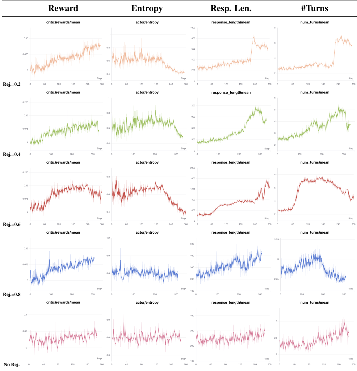
Figure 5: Training dynamics of AGENTICRAG-R1 during GRPO optimization on Qwen2.5-3B under different rejection ratios.
