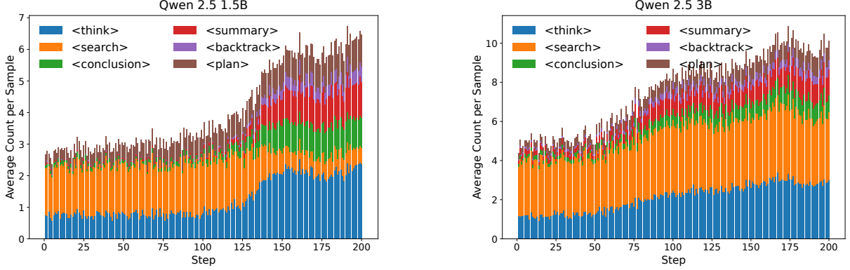
Figure 3: Action-level frequency distributions during RL training across training steps.
