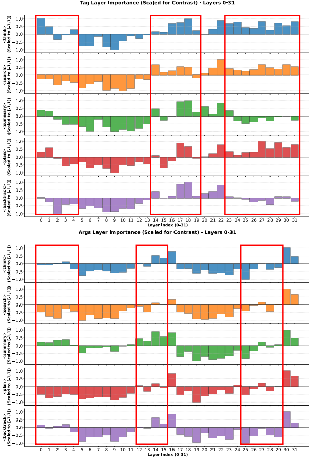
Figure 7: Layer-wise importance profiles of action tokens and their argument tokens.
