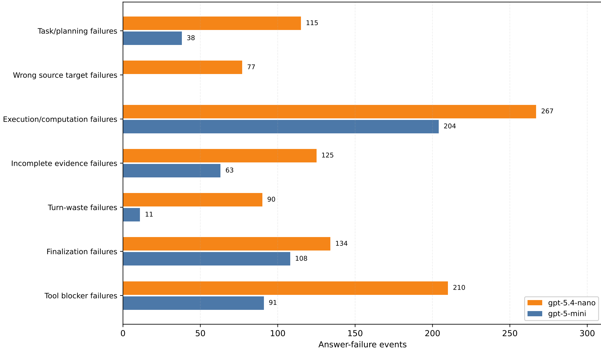
Answer-Failure Groups by Model
